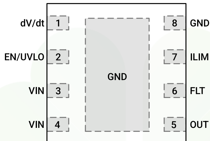
Top View (RS31211A/B, RS31212A/B, RS31309A/B, RS31311A/B)
