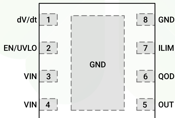
Top View (RS31211D, RS31212D)
